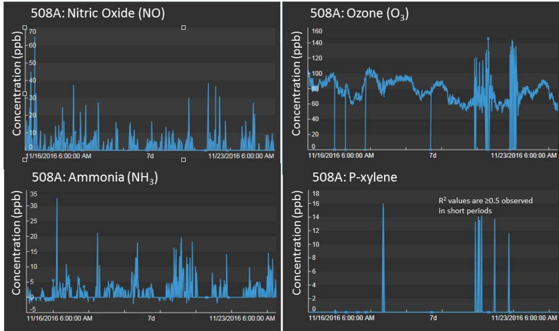
Figure 1. Concentrations of Chemicals Detected by UV-DOAS (508A).
