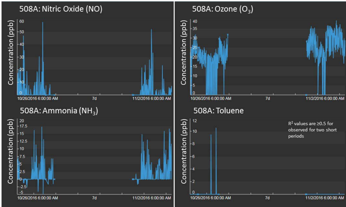
Figure 1. Concentrations of Chemicals Detected by UV-DOAS (508A).
